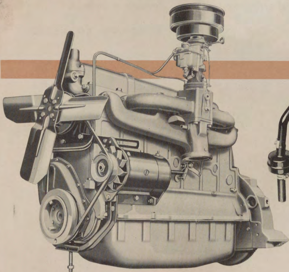
← GMC 270 6-Cylinder Engine 130 H.P. 7.75 to 1 Compression Ratio
