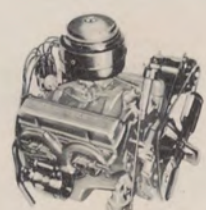
Trademaster V8—155-h.p., 265-cu.-in. displacement, 8 to 1 compression ratio. Optional at extra cost, in Series 3000-4000.
