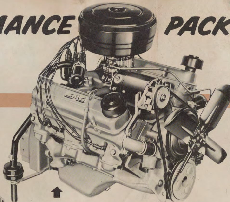
↑ GMC 347 V-8 Engine for Power Plus Performance. 206 H.P. 7.8 to 1 Compression Ratio
