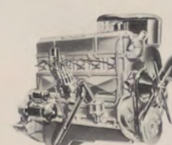
Blue-Flame 140—140 h.p., 235-cu.-in. displacement, 8 to 1 compression ratio. Standard in Sedan Delivery.
