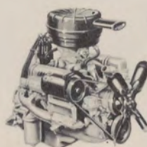
Super Loadmaster V8—210-h.p., 322-cu.-in. displacement, 7.7 to 1 compression ratio. Optional at extra cost in Series 9000-10000.
