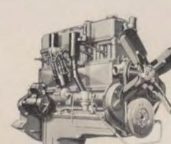
Thriftmaster Special 6—140 h.p., 235-cu.-in. displacement, 8 to 1 compression ratio. Standard in Models 3442, 3542, 3742.
